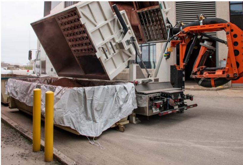
Dry material is dumped into on site bins, and removed from site while truck continues to work.
